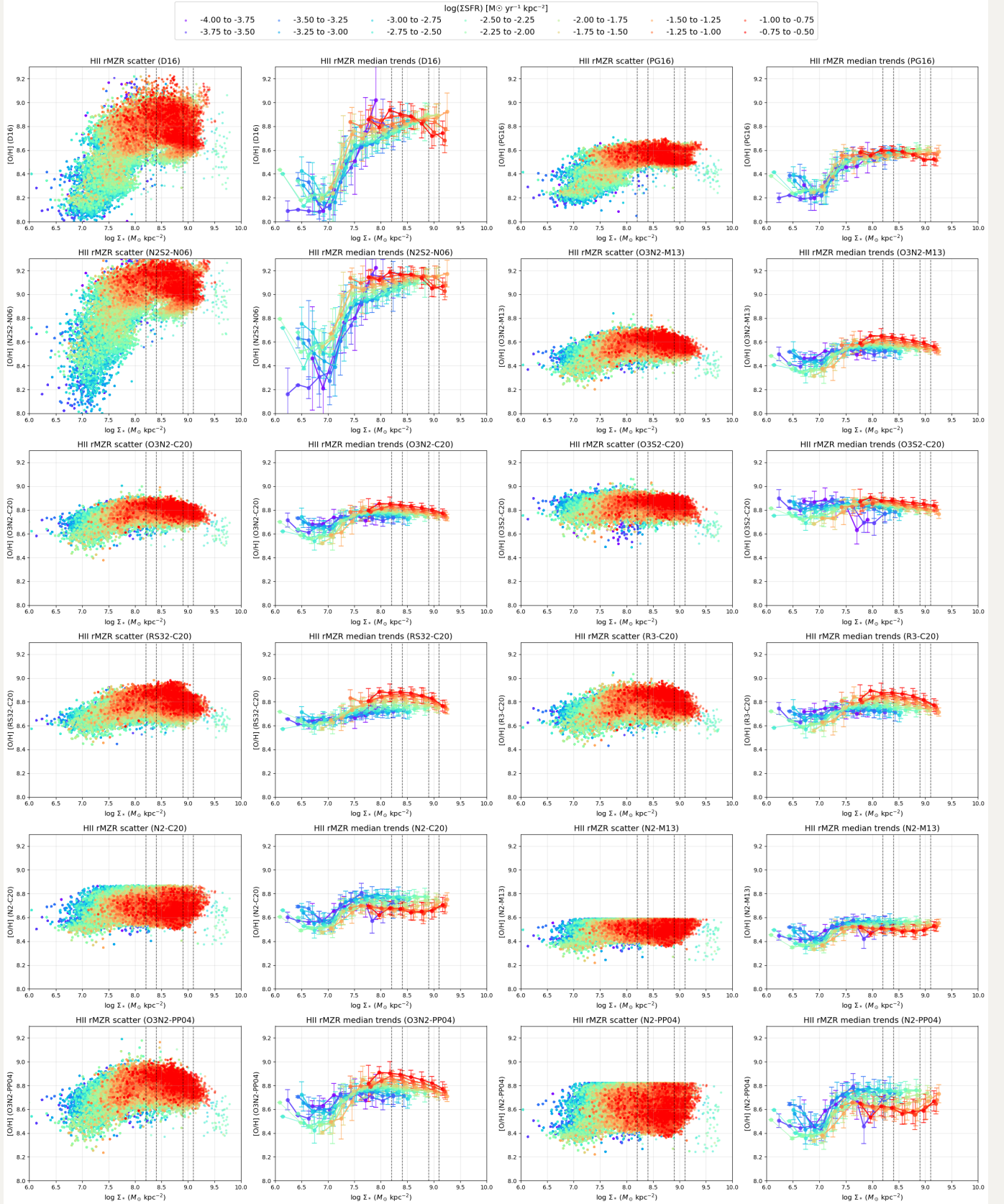
rMZR behavior in \Sigma_{\text{SFR}} bins: HII regions only, No {'NGC4383'} (Min 50 datapoints, Adjacent bins only)
