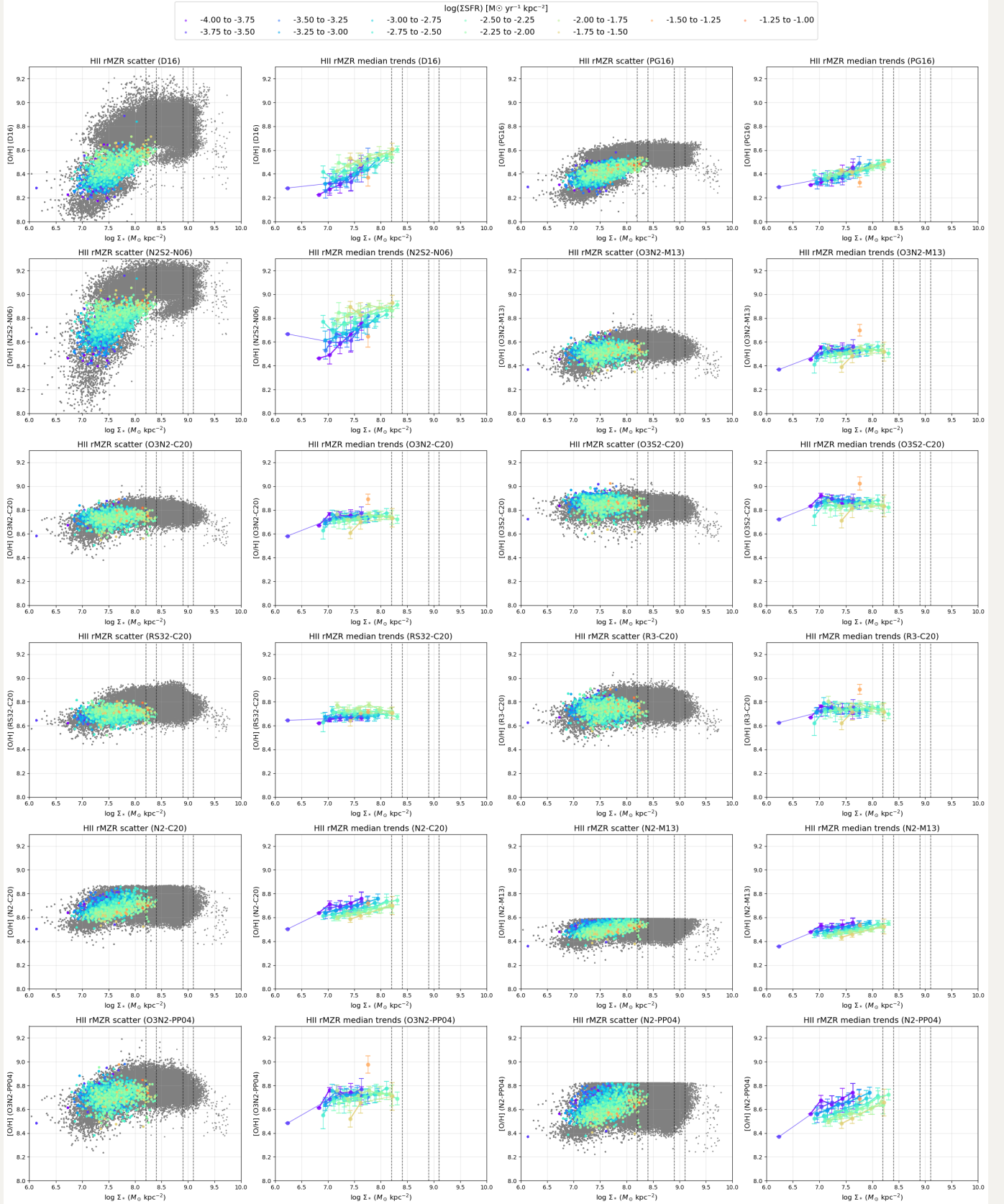
NGC4330: rMZR behavior in \Sigma_{\text{SFR}} bins - HII regions only (Min 50 datapoints, Adjacent bins only)
