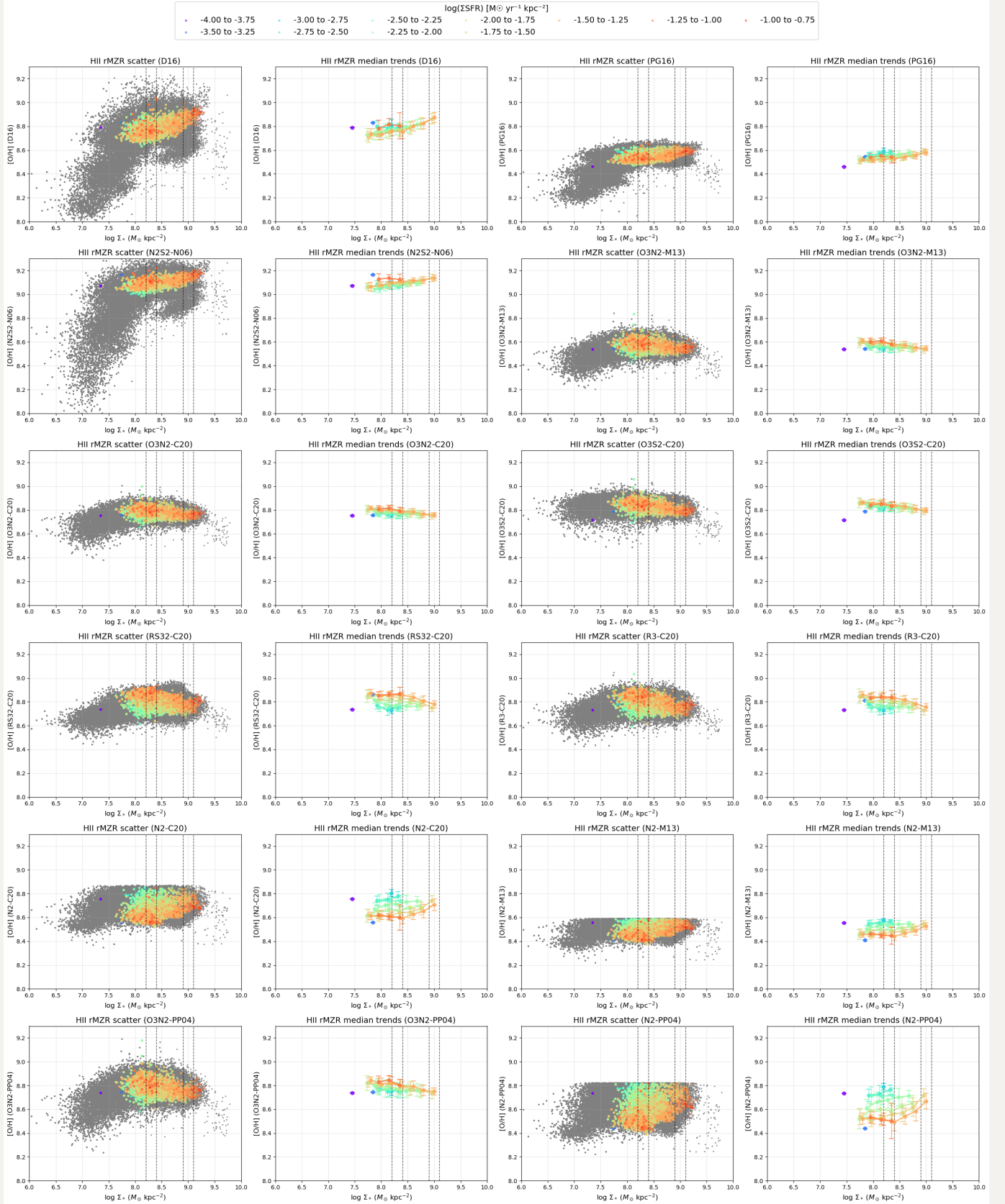
IC3392: rMZR behavior in \Sigma_{\text{SFR}} bins - HII regions only (Min 50 datapoints, Adjacent bins only)
