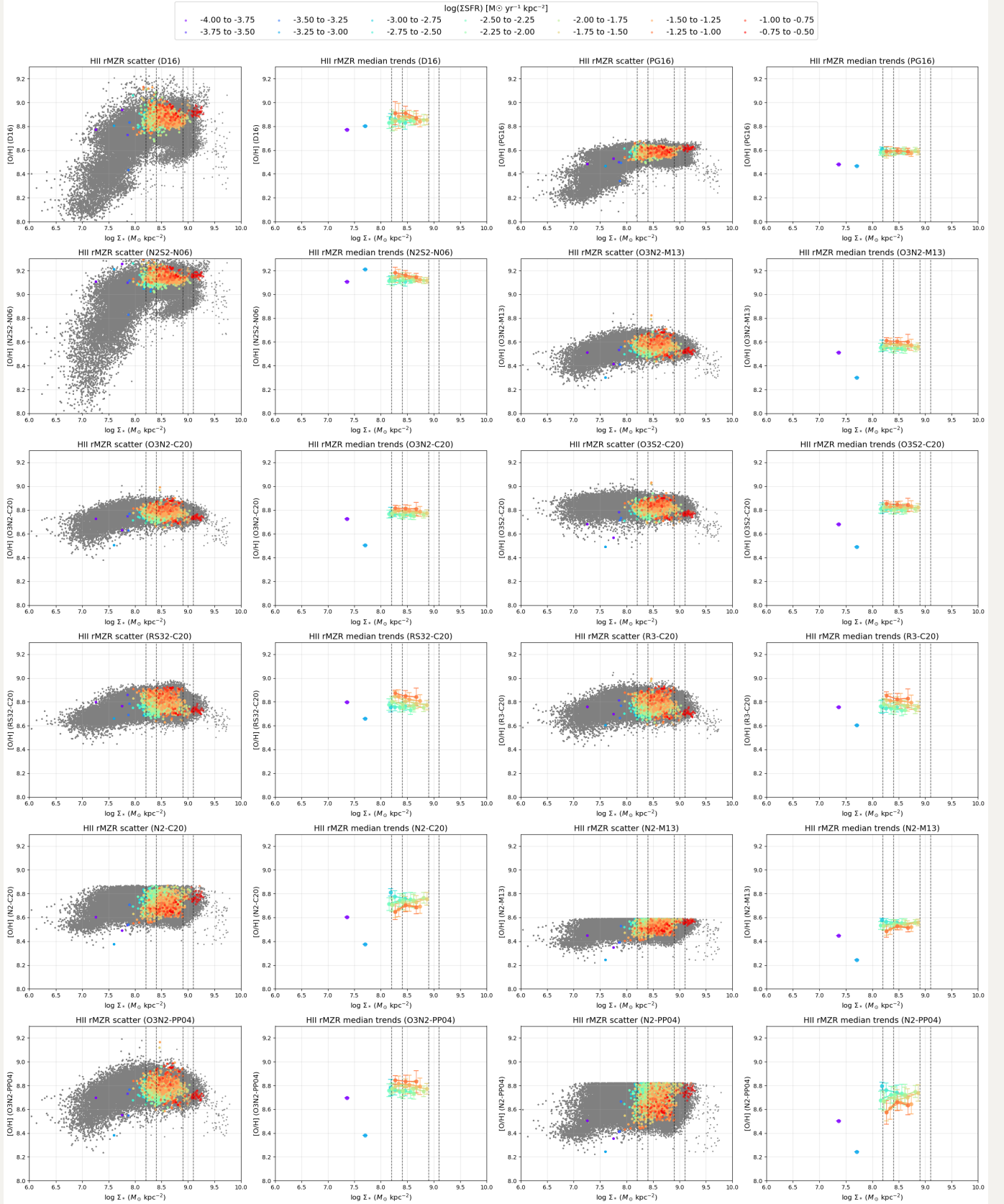
NGC4419: rMZR behavior in \Sigma_{\text{SFR}} bins - HII regions only (Min 50 datapoints, Adjacent bins only)
