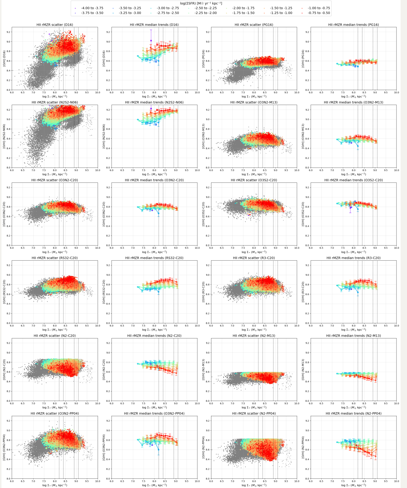
NGC4501: rMZR behavior in \Sigma_{\text{SFR}} bins - HII regions only (Min 50 datapoints, Adjacent bins only)
